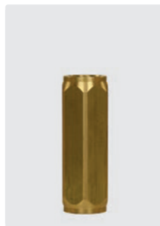
3/8" F. Brass. I 65 mm. Opening pressure 0.05 - 0.1 bar. Max. 150 bar / 90 °C
