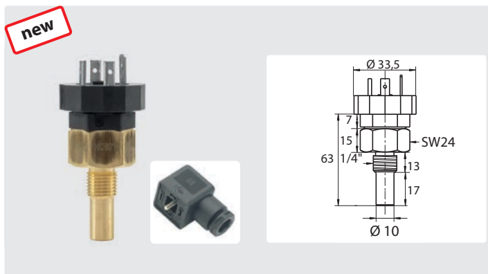
Bimetal temperature switch with plug. Switching point accuracy \pm 5^{\circ}\text{C} . Reset temperature 15...40K. Switching voltage up to AC 250 V / 2A. Max. 10 bar in the inlet. Switch 1/4" M
